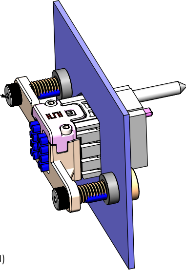
FIG 5 TORQUE SCREWS (NVCF-XX-04-V-X-XX-2-X-X-X-X SHOWN)
