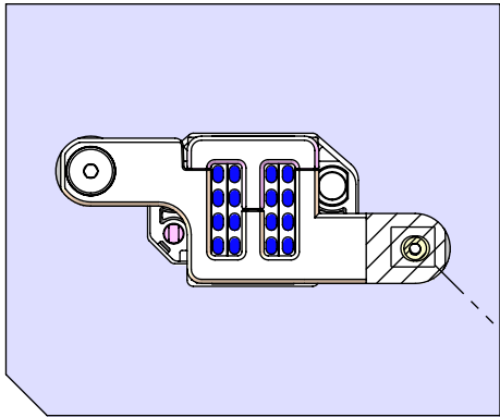
04-12 ROWS, SIDE LUG MOUNTING STYLE (NVCF-XX-04-V-X-XX-2-X-X-X-X SHOWN)
