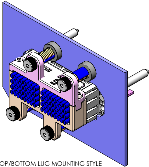
16-32 ROWS, TOP/BOTTOM LUG MOUNTING STYLE (NVCF-XX-16-V-X-XX-9-X-X-X-X SHOWN)
